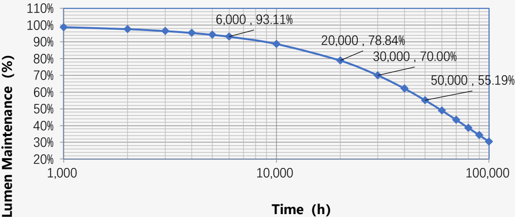
Lumen Maintenance Curve (Percentage of Initial Luminous Flux)
